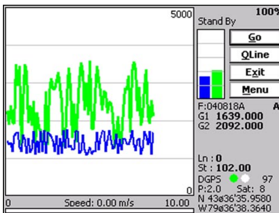
Figure 8.21: The NAV601 screen in the Stand By mode and Profile display mode
