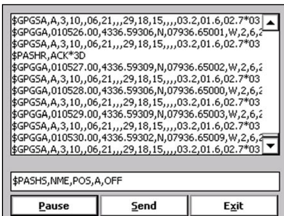
Figure 6.11: GPS Monitoring screen after NMEA command is sent
