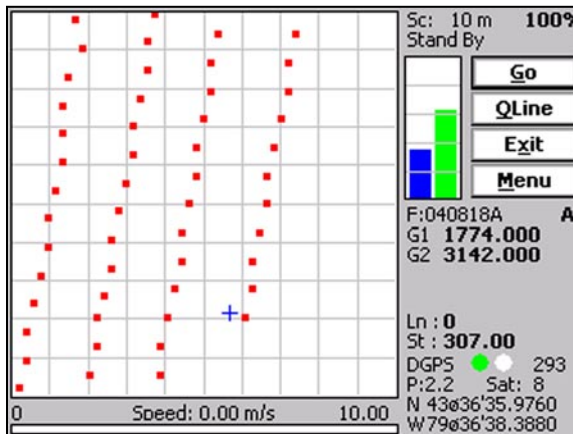
Figure 8.31: The NAV601 screen in Navigation mode after change of map scale
