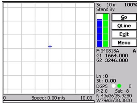
Figure 8.3: Logging screen in Monitoring (Navigation) mode
