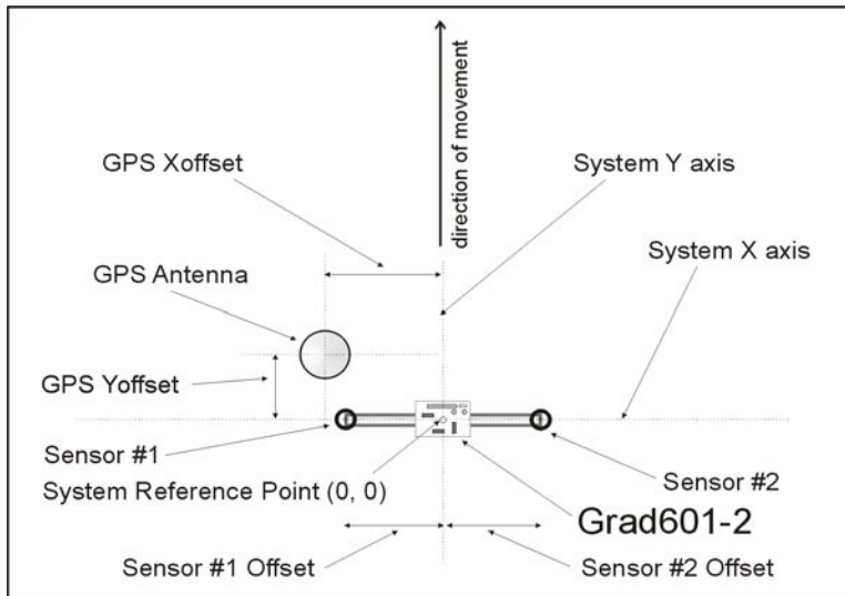
Figure 1.7: The NAV601 system geometry
