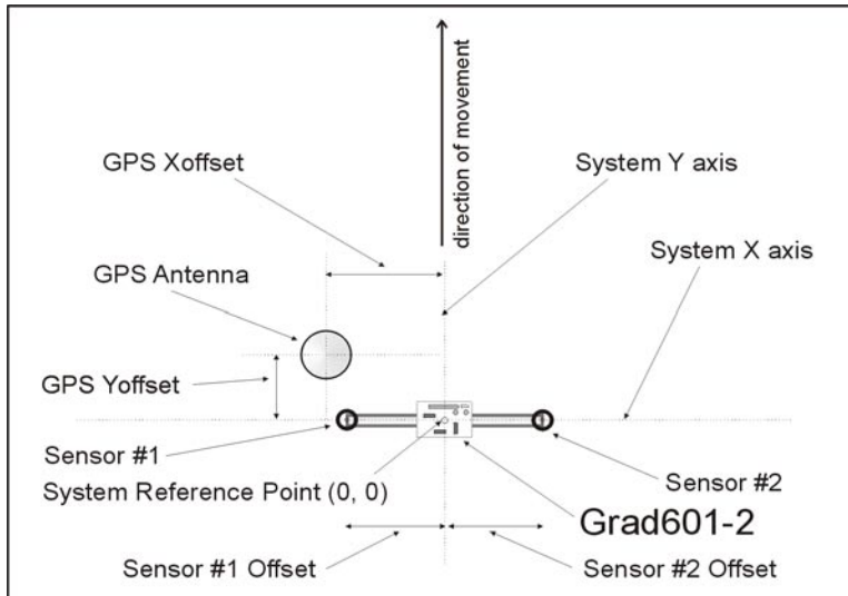
Figure 4.3: Geometry of the instrument and GPS in the field
