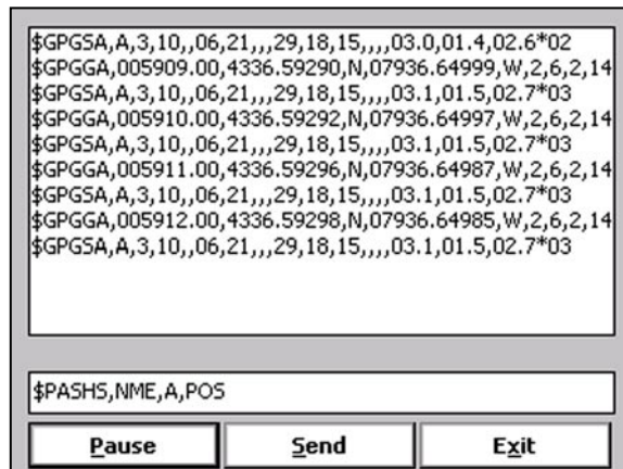
Figure 6.6: Monitoring GPS output in monitoring (terminal) mode
