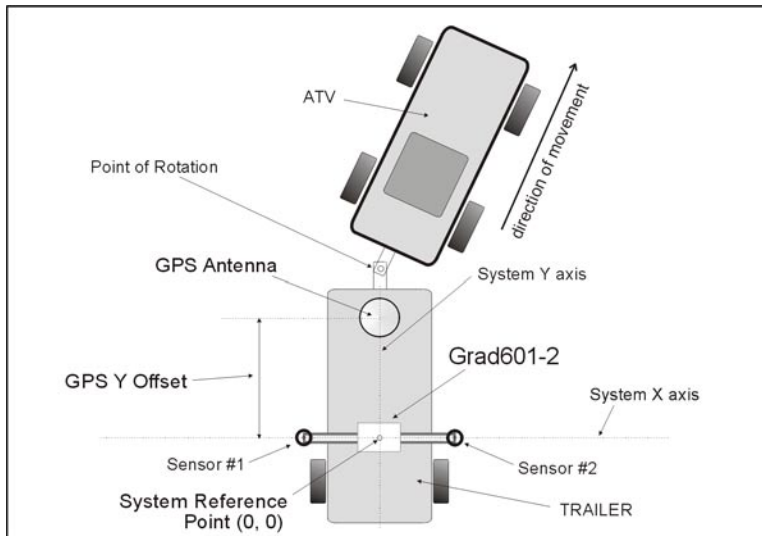
Figure 4.4: Geometry of the Grad601 and GPS antenna during towing
