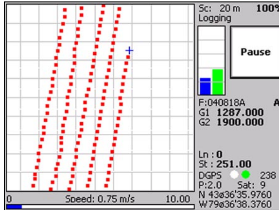
Figure 8.22: The NAV601 screen in Logging mode (Navigation display mode)
