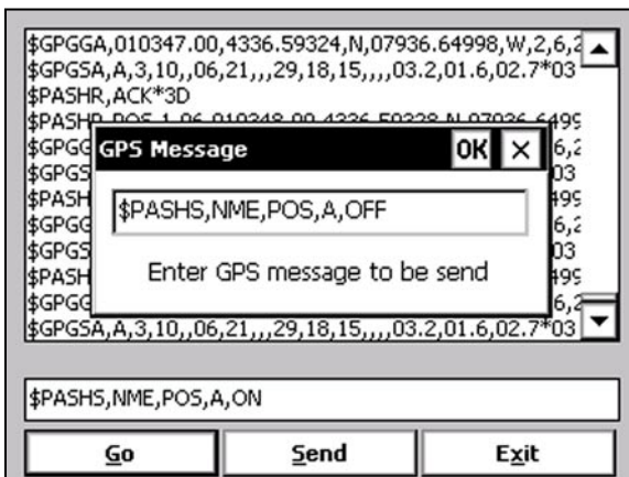
Figure 6.10: Example of the NMEA command entry
