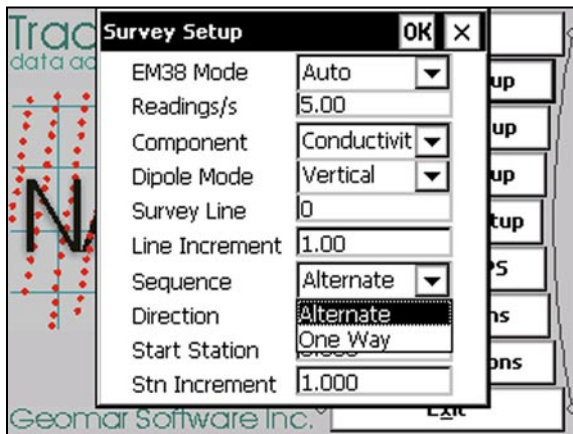
Figure 3.4: Selecting component in Manual mode
