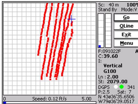
Figure 8.33: The NAV38 screen in Navigation mode after change of map scale
