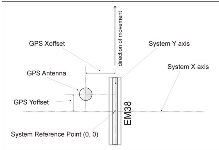
Figure 1.5: The NAV38 system geometry
