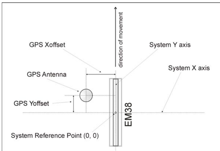
Figure 4.2: Geometry of the instrument and GPS in the field
