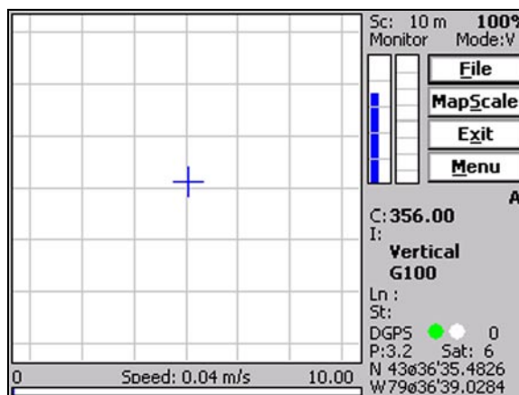
Figure 8.1: Initial NAV38 Monitoring screen in Navigation mode
