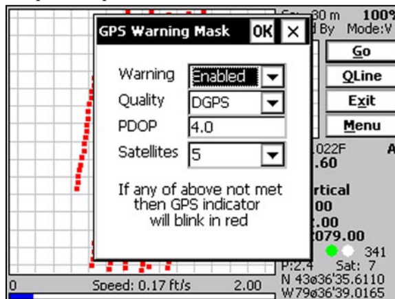
Figure 8.37: GPS Warning Mask dialog
