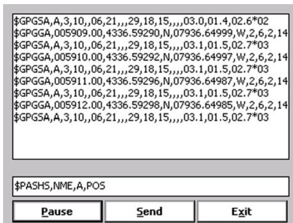
Figure 6.5: Monitoring GPS output in monitoring (terminal) mode
