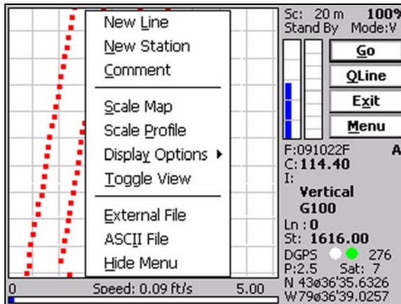
Figure 8.26: List of items in pop up menu in Stand By mode
