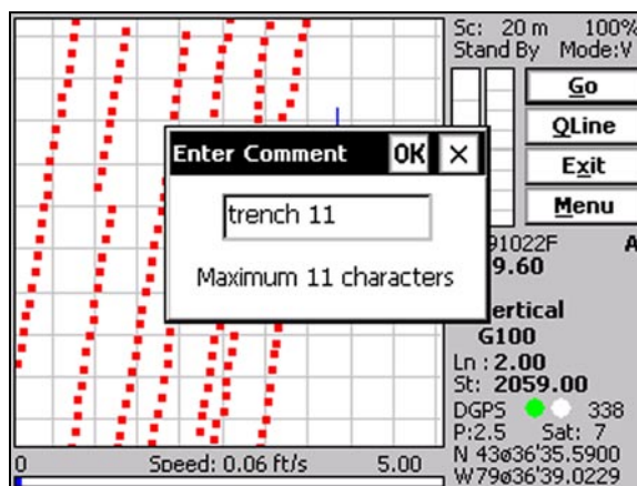
Figure 8.31: Enter Comment dialog
