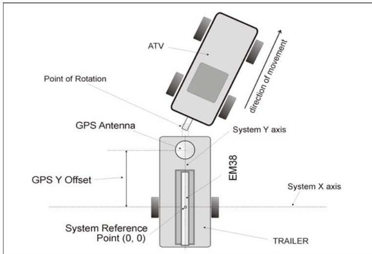
Figure 4.3: Geometry of the EM38 and GPS antenna during towing
