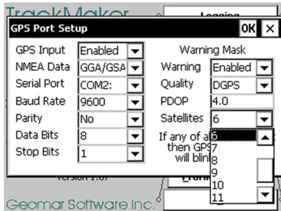
Figure 6.4: Selecting minimum number of satellites
