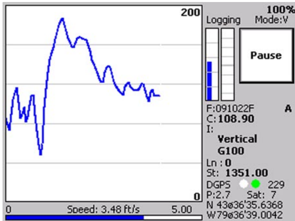
Figure 1.4: The NAV38 in the Profile mode
