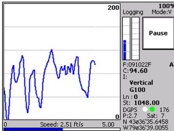
Figure 7.7: NAV38 in Profile Display mode and conductivity scale grid lines
