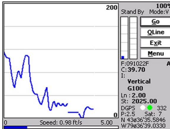
Figure 8.30: Profile display after New Station was entered
