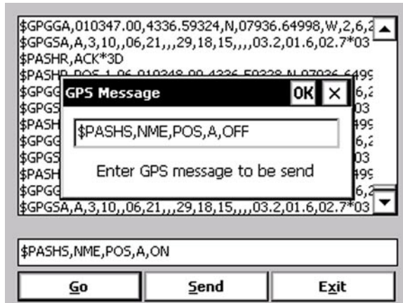
Figure 6.9: Example of the NMEA command entry
