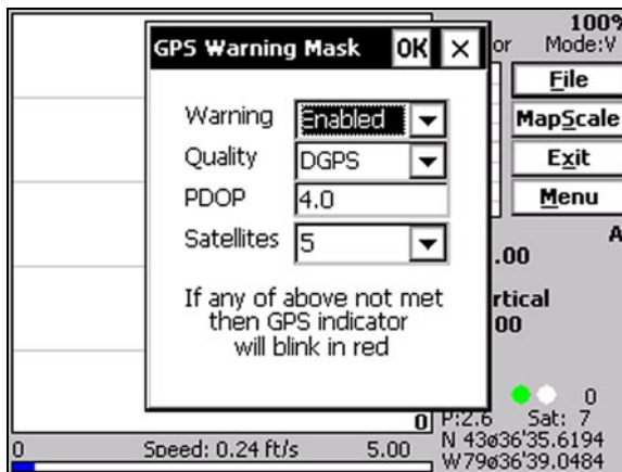
Figure 8.12: GPS Warning Mask dialog
