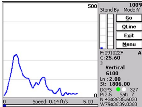
Figure 8.35: Profile display in new scale (compare with Figure 8.34)
